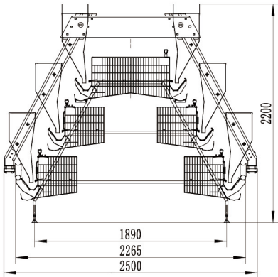
A380 3-storey stepped road-feed laying cage Free drop manure, optional cleaning belt
